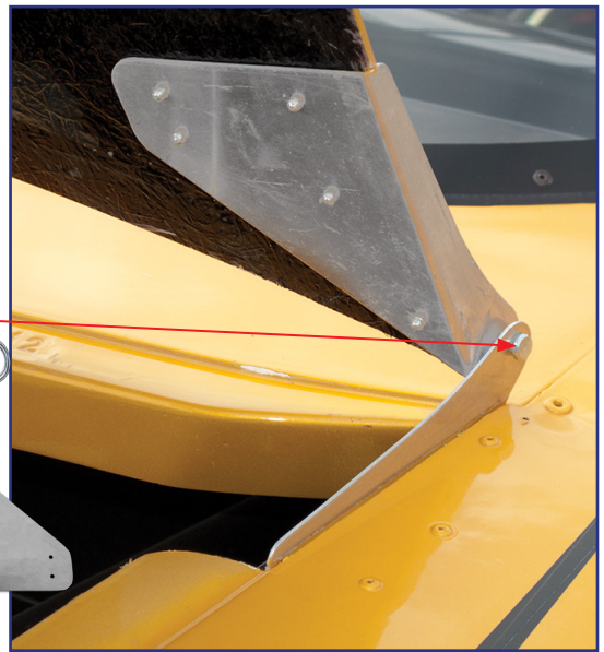
FULLY INSTALLED 000-33H
